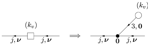
Fig. 7. The quantity \mu^{(k_v)} appearing in the node factor associated with v can be expressed according to (3.10). This can be interpreted graphically by replacing the white square as shown in the figure: the graph element entering the node v represent \mu^{(k_v)} , and it can be further developed in terms of trees according to Fig. 3.
