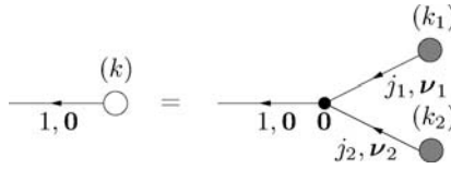
Fig. 4. Graphical representation of (3.12), expressing the constant a_0^{(k)} (hence j = 1 ) for k \geq 2 in terms of the coefficients u_{j', \nu'}^{(k')} , with k' < k . One has the constraints \mathbf{0} = \mathbf{v}_1 + \mathbf{v}_2 , k = k_1 + k_2 , and j_1 = j_2 \in \{1, 2\} .
