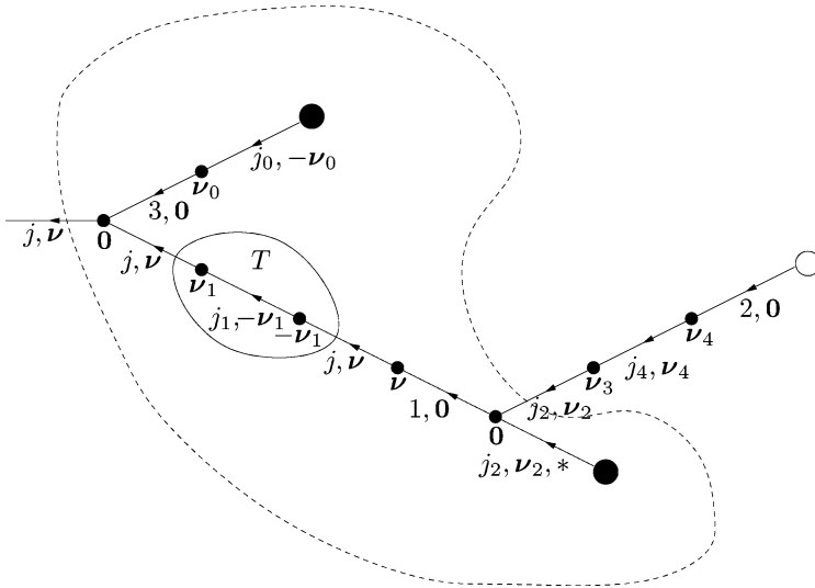
Fig. 10. Example of self-energy cluster. Let T be the set of nodes and lines inside the solid line, i.e. the set consisting of the line \ell with momentum -\nu_1 and of the two nodes \nu_1 and \nu_2 , with mode labels \nu_1 and -\nu_1 , respectively, connected by such a line. Then T is a self-energy cluster if the scale of the line \ell is strictly less than the scales of both the line \ell_2 entering \nu_2 and the line \ell_1 exiting \nu_1 , i.e. if n_\ell < \min\{n_{\ell_1}, n_{\ell_2}\} . In such a case \ell_1 and \ell_2 become the external lines of T . The set of nodes and lines inside the dotted line cannot be a self-energy cluster, even if it is a cluster and \nu = \nu_2 , because the path of lines between the external lines contains a line with vanishing momentum.
