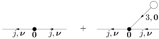
Fig. 12. Self-energy clusters on scale -1 contributing to \mathcal{M}_j^{[\leq n]}(\omega \cdot \nu) . The external lines do not belong to the self-energy clusters, and have been drawn only to help visualising the structure of the self-energy clusters.
