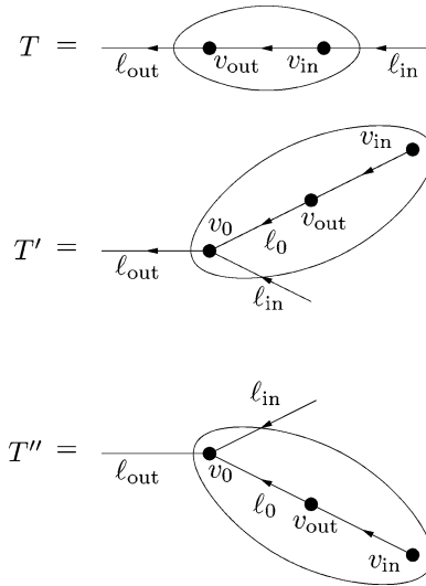
Fig. 11. Examples of renormalised self-energy clusters belonging to the same equivalence class: T is a renormalised self-energy cluster of the second type, while T' and T'' are renormalised self-energy clusters of the first kind. The self-energy values of T' and T'' are equal to each other: in fact the trees containing such renormalised self-energy clusters can be obtained from each other by permuting the entering lines of v_0 . The external lines \ell_{in} and \ell_{out} do not belong to the self-energy clusters, and have been drawn only to help visualising the structure of the self-energy clusters.
